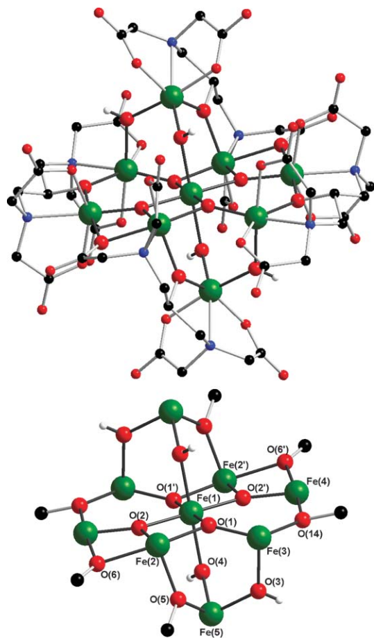
Fig. 2 Structure of the \text{Fe}_9 aggregate 1 in \text{K}_5[\text{I}]\cdot 5\text{MeOH}\cdot 5\text{H}_2\text{O} (above) and the aggregate core (below). Colour code: Fe, green; O, red; N, blue; C, black; H, white. \text{Fe}-(\mu_3\text{-O}) 1.837(3)–2.013(3) Å, \text{Fe}-(\mu\text{-O}) 1.938(4)–2.083(4) Å. Angles at O ( ^\circ ): \text{Fe}(1)\text{-O}(1)\text{-Fe}(2) 96.0(1), \text{Fe}(1)\text{-O}(1)\text{-Fe}(3) 129.2(2), \text{Fe}(2)\text{-O}(1)\text{-Fe}(3) 128.8(2), \text{Fe}(1)\text{-O}(2)\text{-Fe}(2) 97.4(1), \text{Fe}(1)\text{-O}(2)\text{-Fe}(4') 150.4(2), \text{Fe}(2)\text{-O}(1)\text{-Fe}(4') 112.2(2), \text{Fe}(3)\text{-O}(3)\text{-Fe}(5) 123.8(2), \text{Fe}(1)\text{-O}(4)\text{-Fe}(5) 124.5(2), \text{Fe}(2)\text{-O}(5)\text{-Fe}(5) 120.2(2), \text{Fe}(2)\text{-O}(6)\text{-Fe}(4') 95.0(1), \text{Fe}(3)\text{-O}(14)\text{-Fe}(4) 128.5(2).
