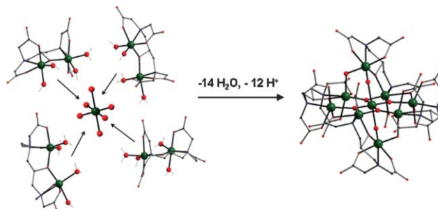
Fig. 1 Formal hydrolytic encapsulation of [\text{Fe}(\text{H}_2\text{O})_6]^{3+} by four \{\text{Fe}_2(\text{hpdt})(\text{H}_2\text{O})_4\}^+ species to give [\text{Fe}_9(\mu_3\text{-O})_4(\mu\text{-OH})_4(\text{hpdt})_4]^{5-} .
