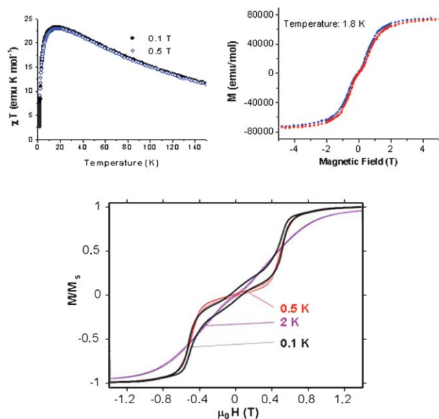
Fig. 3 Magnetic properties of K_5[1] \cdot 5H_2O \cdot 5CH_3OH ; \chi T vs. T (top, left), field dependence of the magnetisation at 1.8 K (top, right), \mu -SQUID measurements on a single crystal at 2 K, 0.5 K and 0.1 K (below).
